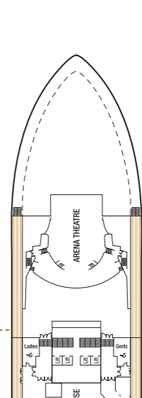
DECK 7 - PROM DECK
